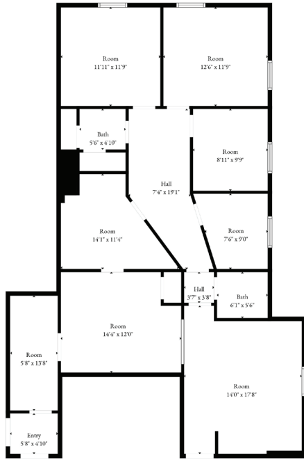
A3 Floor Plan
